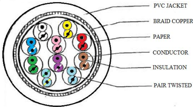
Cable Construction
