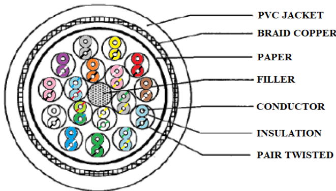
Cable Construction
