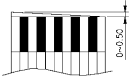
Tolerance of Cutting Tilt
