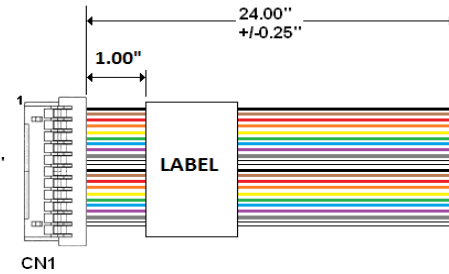
QD10781 DISCRETE WIRE FLYING LEAD ASSY
