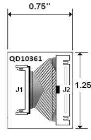
QD10361 PCB ADAPTER
