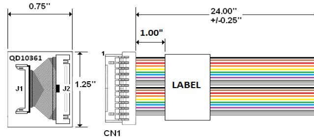
QD10361 PCB ADAPTER QD10781 DISCRETE WIRE FLYING LEAD ASSY LABEL = QD# + CODE
