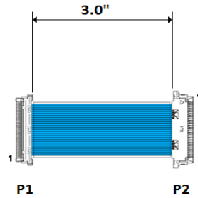
SGC1018 SMALL GAUGE COAX JUMPER
