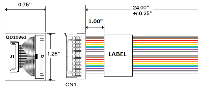
QD10361 PCB ADAPTER QD10781 DISCRETE WIRE FLYING LEAD ASSY
