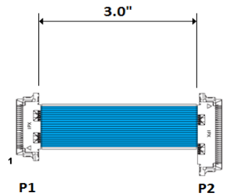
SGC1004 SMALL GAUGE COAX JUMPER
