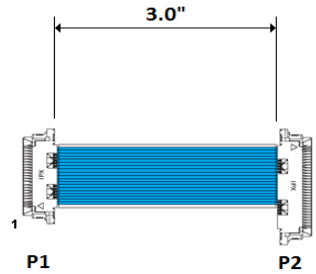
SGC1002 SMALL GAUGE COAX JUMPER
