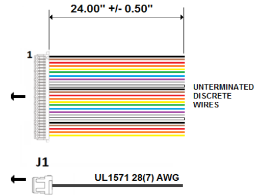
DISCRETE WIRE CABLE SECTION
