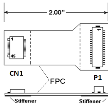
FPC SECTION
